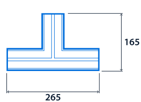
Tee Joint
