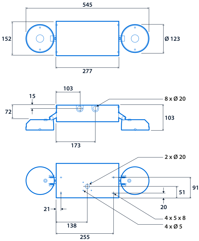
IP20 version
