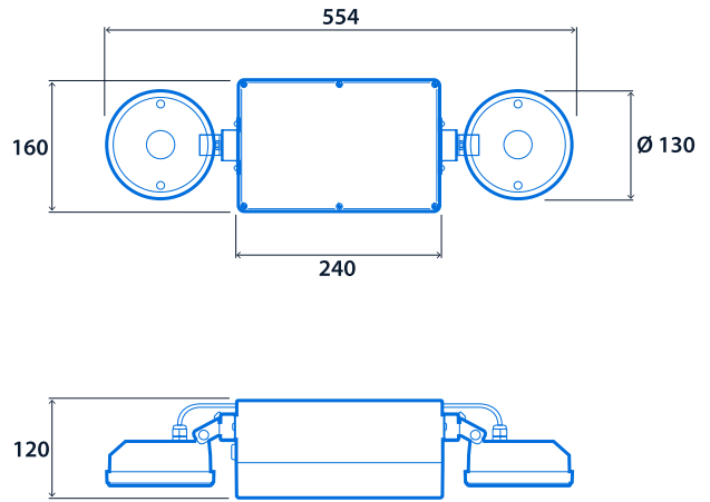
IP65 version
